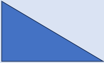
Triangle rectangle
