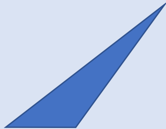
Triangle quelconque
